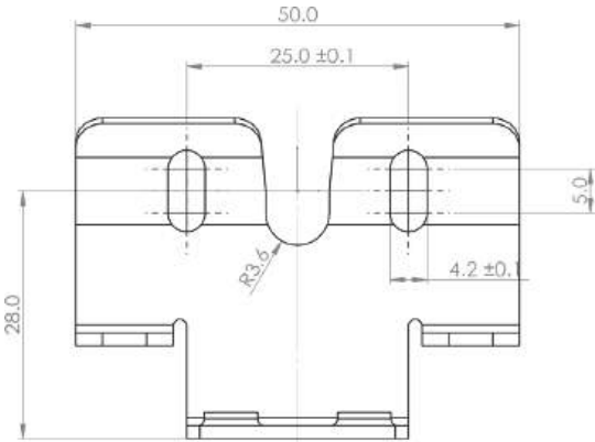
FLEX-180-L
