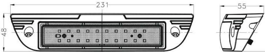
CSSL-20-XR
