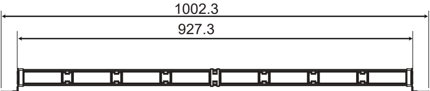
Focus 800
