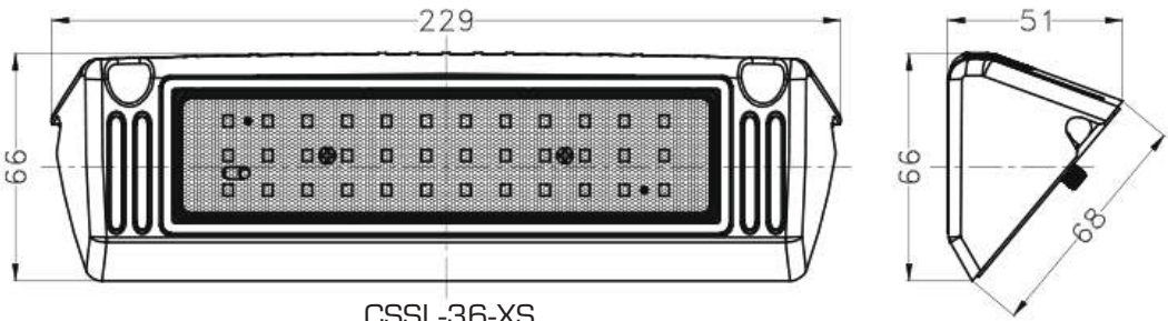
CSSL-36-XS
