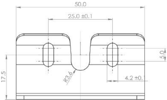
FLEX-180-C
