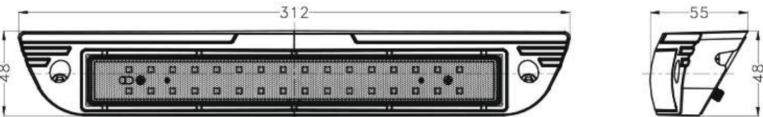
CSSL-32-XR
