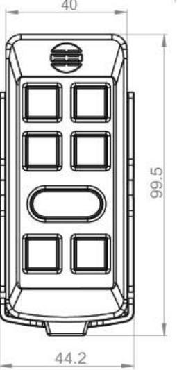
CONTROLLER
